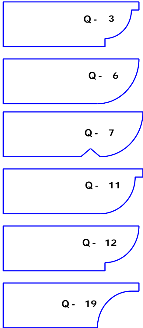
Standard QuattroCorbel Profiles Custom Profiles Available Upon Request
